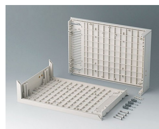
B201117 L-shells D 160, with holes for handle ABS (UL 94 HB) off-white RAL 9002 290x200x74mm
