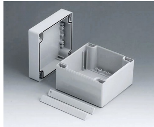
C2112122 ROBUST-BOX 120 BREIT, Ausf. II PC (UL 94 HB) lichtgrau RAL 7035 120x120x90mm IP 66
