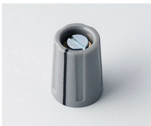
A2610038 ROUND KNOB 10, with line ABS (UL 94 HB) dusty grey RAL 7037 10x14mm 3mm
