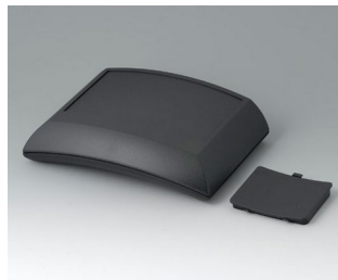
B7020109 ERGO-CASE L, plate ABS (UL 94 HB) noir RAL 9005 150x200x54mm IP 54 opt.
