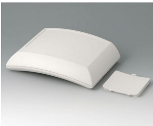
B7020107 ERGO-CASE L, plate ABS (UL 94 HB) gris blanc RAL 9002 150x200x54mm IP 54 opt.
