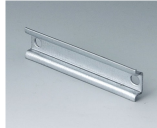
C7110087 Standard DIN rail, Type TH 15 Steel 66x15x5,5mm
