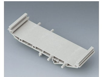
B6724443 RAILTEC SUP. 107, intermediate part + foot PA 6 (30) (UL 94 V-0) light grey 118x35x27,5mm
