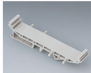
B6724442 RAILTEC SUP. 107, intermediate part + foot PA 6 (30) (UL 94 V-0) light grey 118x18,5x27,5mm
